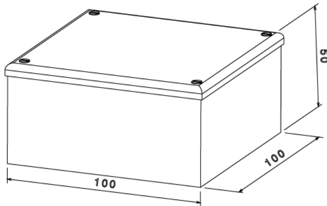
Isometric view
