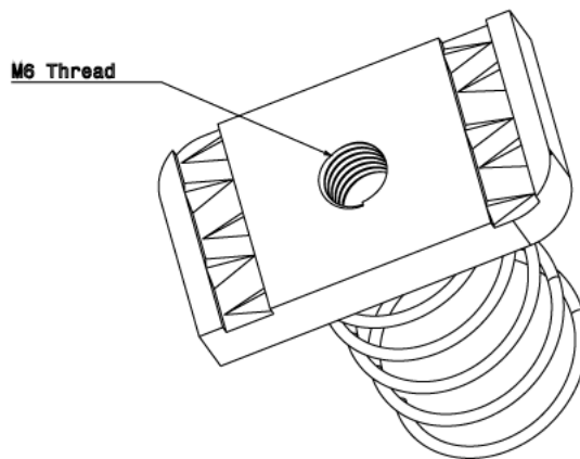
Isometric view
